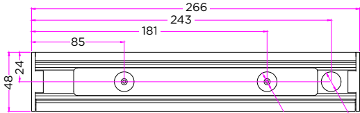
Ø5 FIXING HOLES Ø16 CABLE ENTRY
