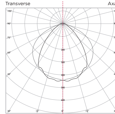
LUMINAIRE LUMEN OUTPUT BROAD 8W = 1035lm
