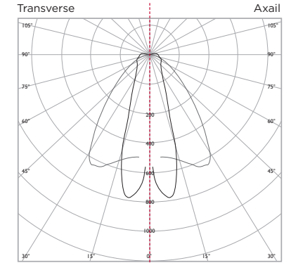
LUMINAIRE LUMEN OUTPUT NARROW 8W = 1025lm
