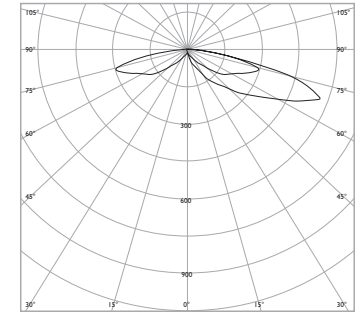
LUMINAIRE LUMEN OUTPUT 5W = 450lm - Path Distribution 11W = 780lm - Path Distribution
