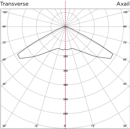
LUMINAIRE LUMEN OUTPUT 4W = 215lm
