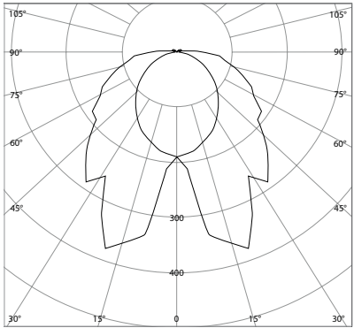
LANT300 LANT300 = 950lm
