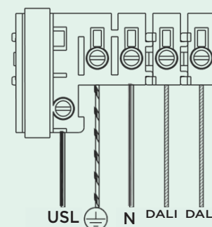
DALI (IP RATED)
