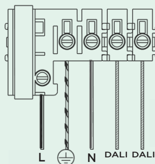
CENTRAL SUPPLY DALI (IP RATED)
